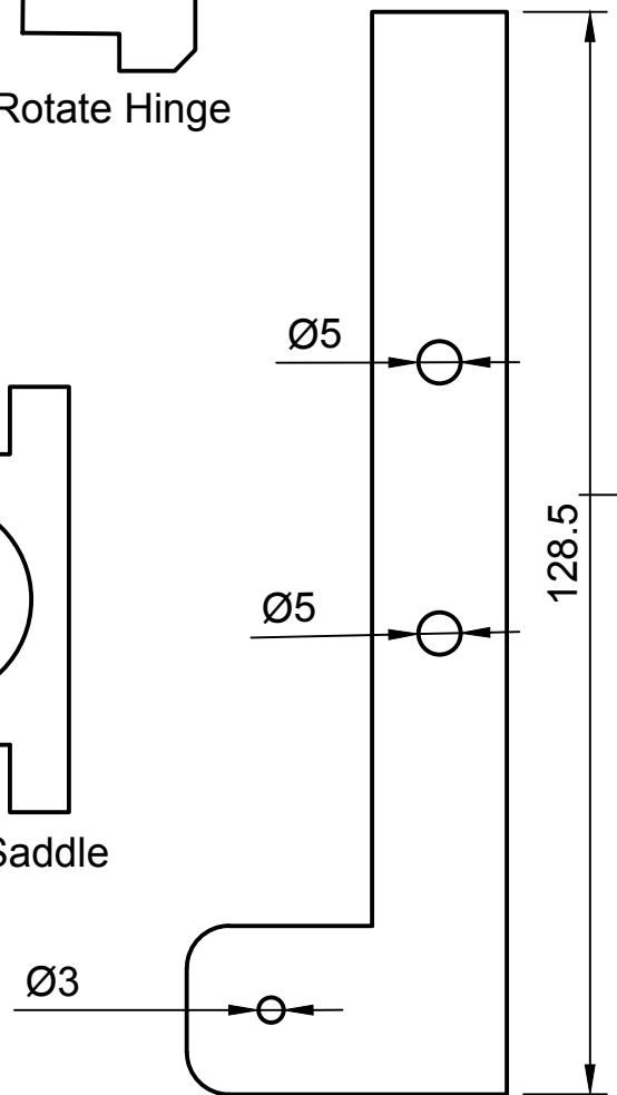
"L" Bracket
